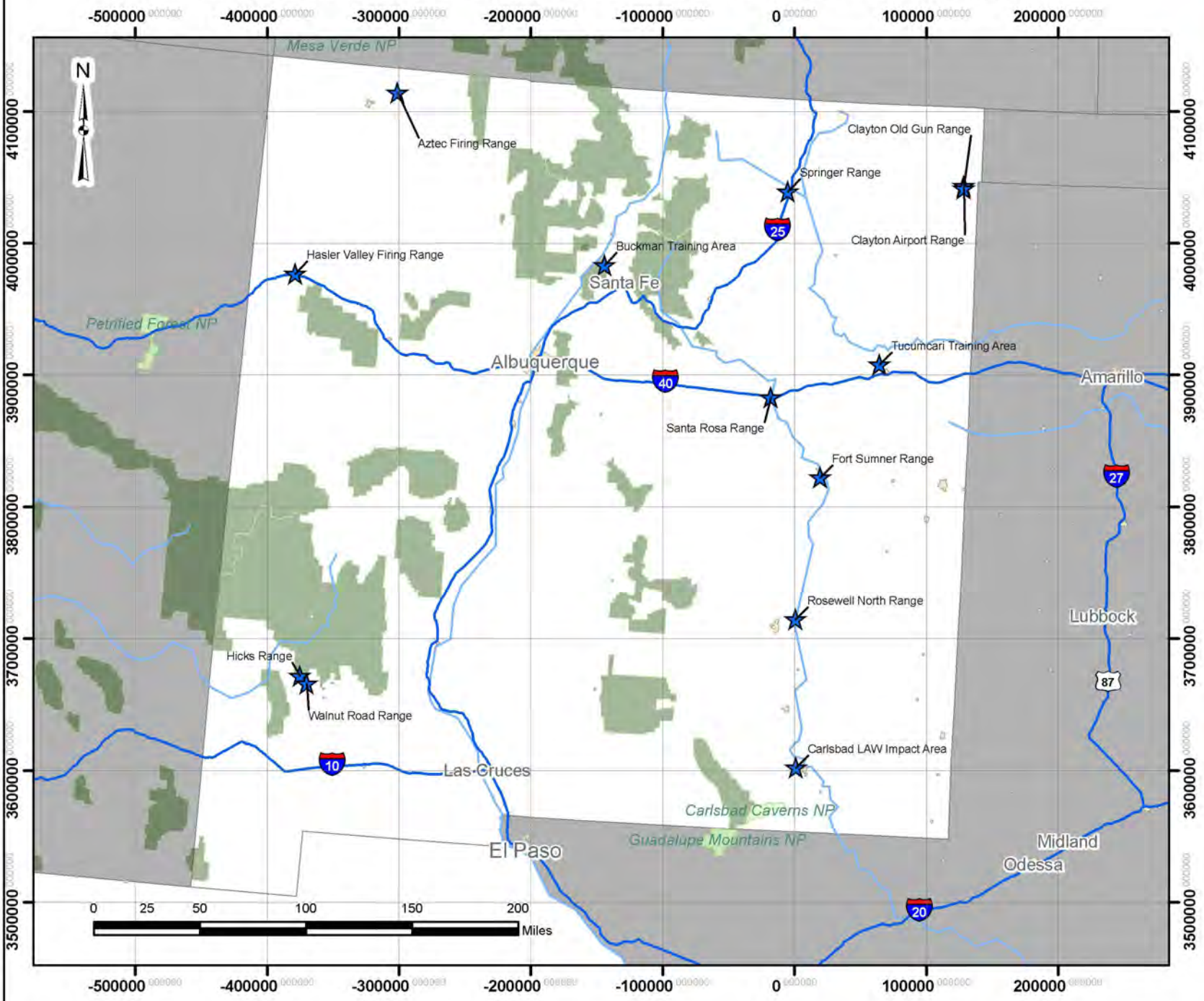
NDNODS Map New Mexico Figure ES-1
